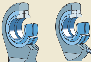
Lubrication hole
